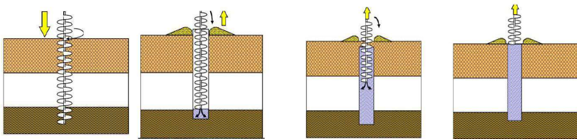
Figure 4.2: CFA Piling Sequence Illustration
